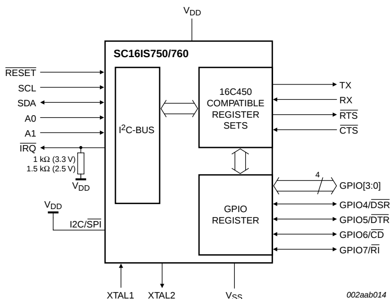
Fig 1. Block diagram of SC16IS750/760 I 2 C-bus interface
