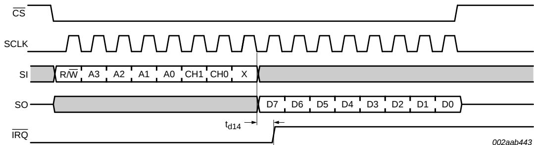
Fig 41. Read RHR to clear RX INT
