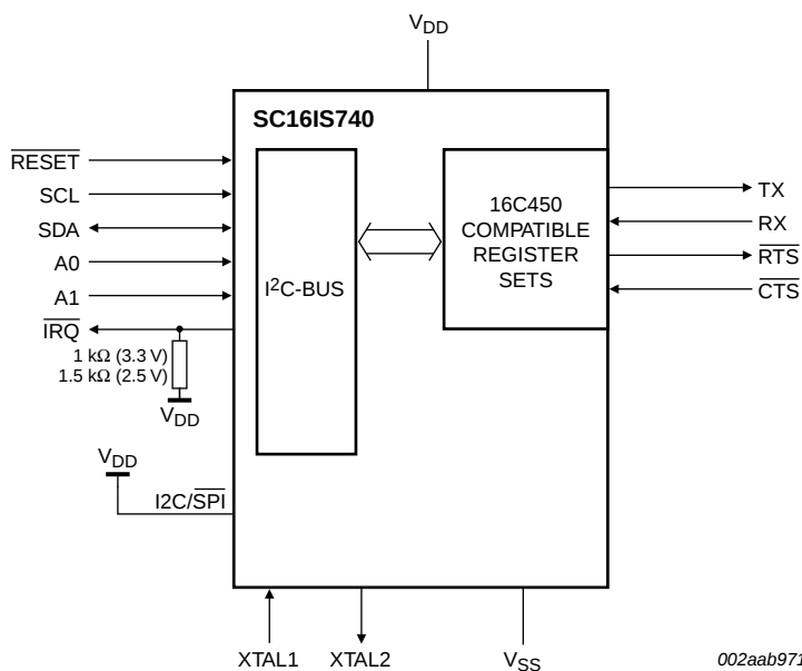
Fig 2. Block diagram of SC16IS740 I 2 C-bus interface
